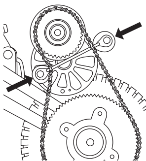
7 Reset chain tensioner.
