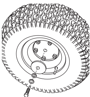
11 On the outside of the wheel replace washers and secure with bolt.
