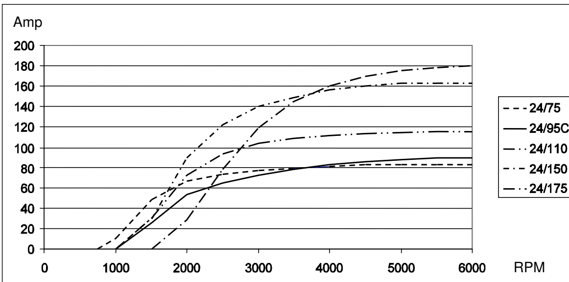
Figure A-15: Characteristics for Mastervolt alternators: charge current versus RPM
