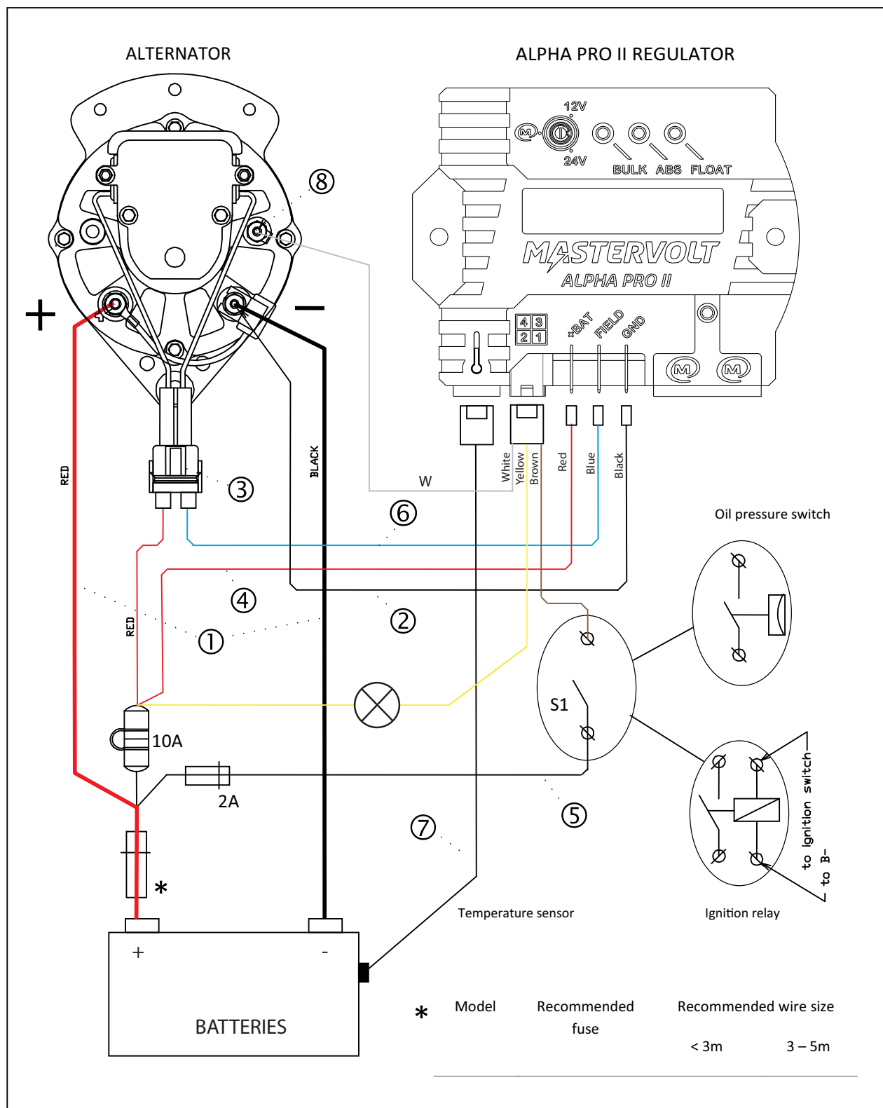
Figure A-6: Installation drawing Alpha alternator model 12/90
