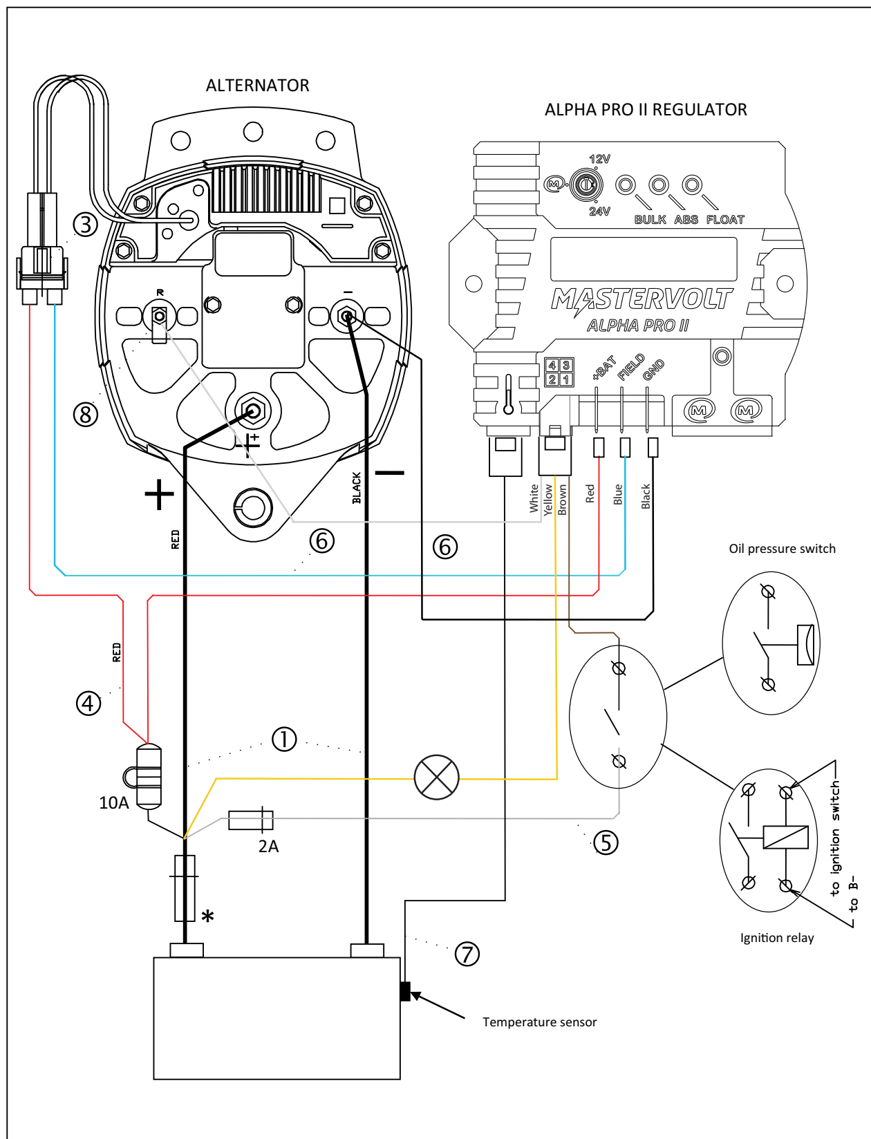
Figure A-8: Installation drawing Alpha alternator model 24/150
