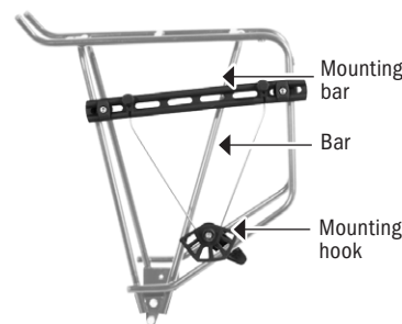
QL3/QL3.1 mounting components (incl.)
