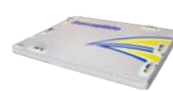
SWIMSTEP™ XL HD L 5' x W 6.5' x H 0.4' (L 1,5m x W 2m x H 0,1m)
