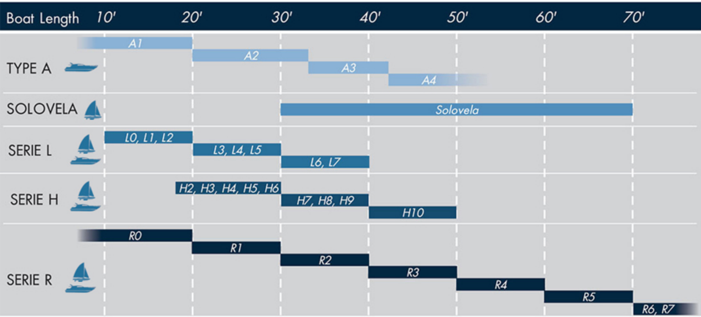
Fenders Selection Chart
